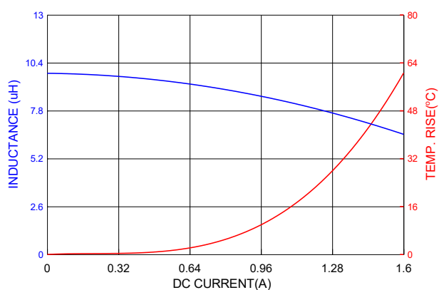
PIC0315H100MF
