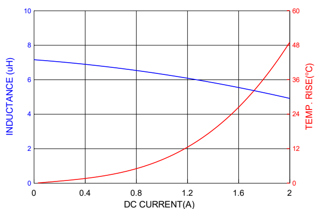
PIC0315H6R8MF
