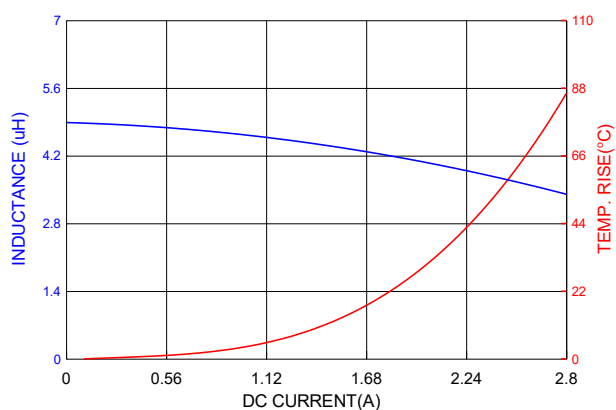
PIC0315H4R7MF
