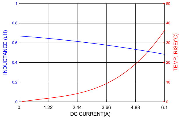
PIC0312HR68MF
