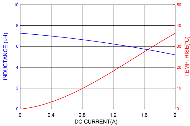
PIC0312H6R8MF
