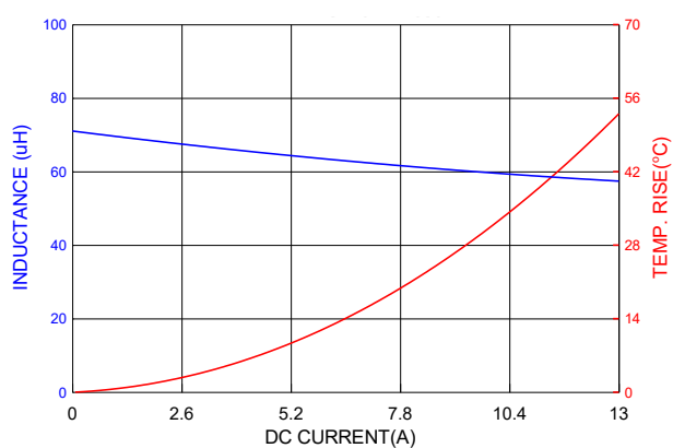
PIC1707HP680MF
