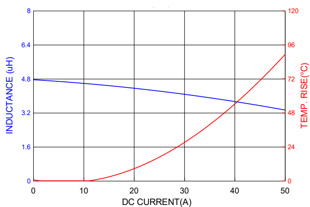
PIC1707HP4R7MF
