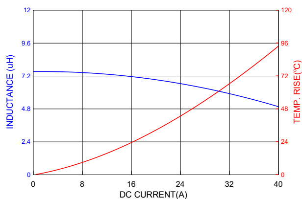
PIC1707HP7R4MF
