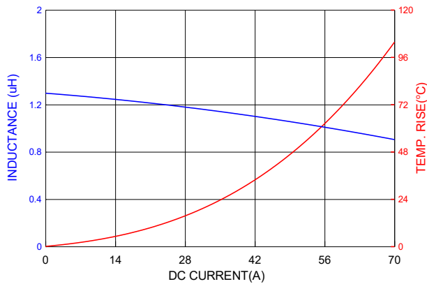
PIC1707HP1R5MF
