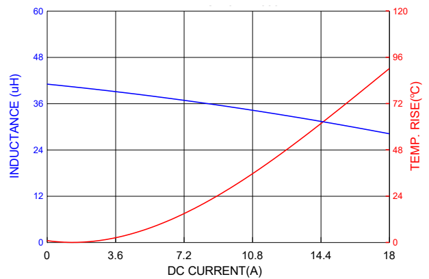
PIC1707HP390MF
