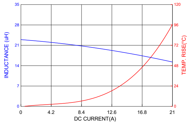
PIC1707HP220MF
