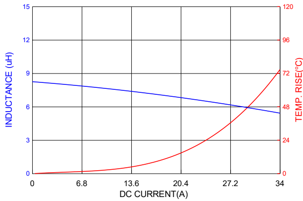
PIC1707HP8R2MF
