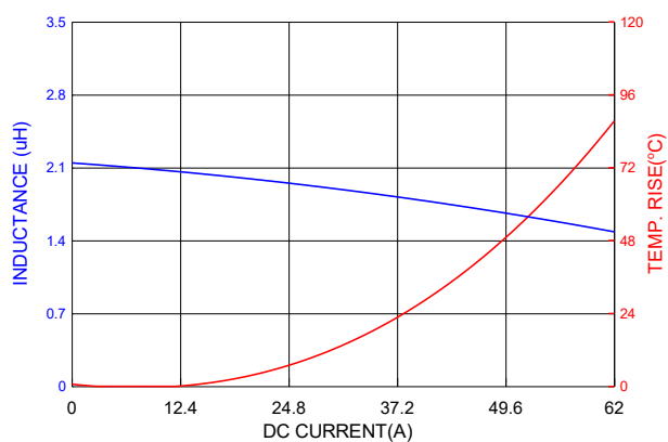
PIC1707HP2R2MF
