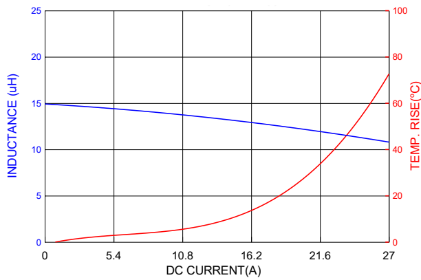
PIC1707HP150MF
