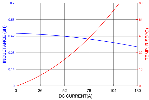
PIC1707HPR45MF
