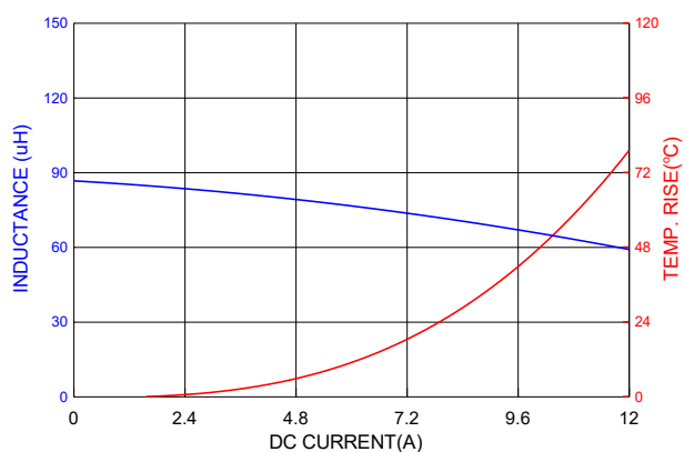
PIC1707HP101MF
