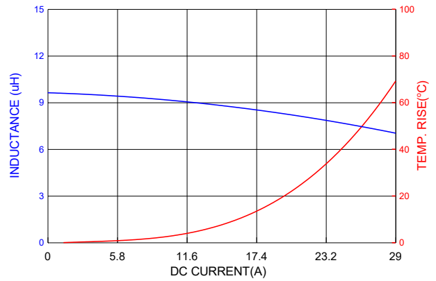
PIC1707HP100MF
