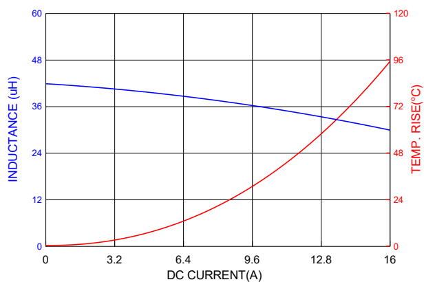
PIC1707HP470MF
