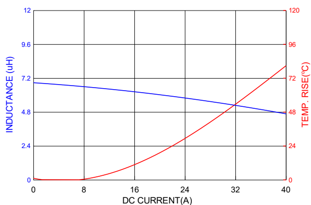
PIC1707HP6R8MF
