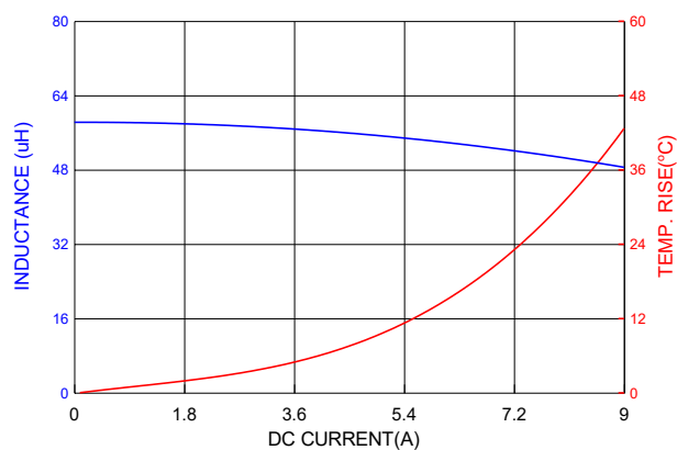
PIC1707HP560MF
