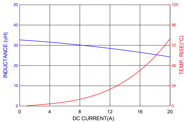
PIC1707HP330MF
