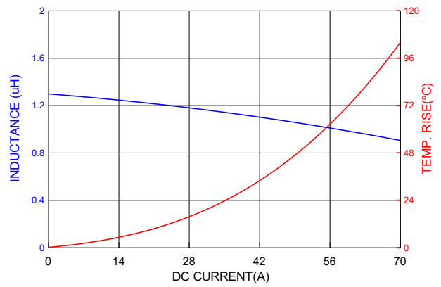
PIC1707HP1R3MF
