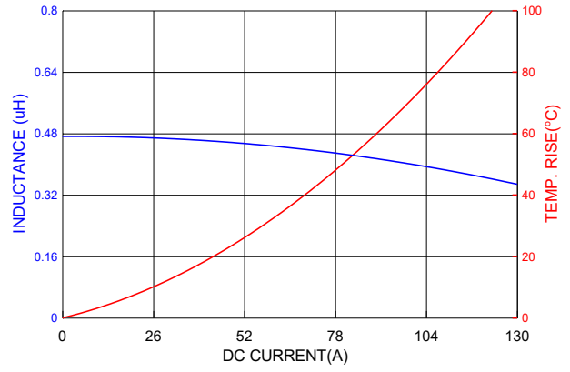
PIC1707HPR47MF
