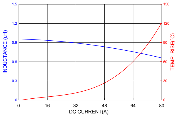
PIC1707HP1R0MF
