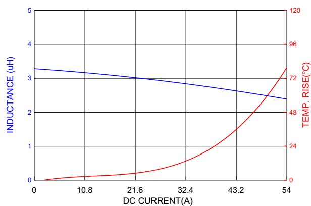
PIC1707HP3R3MF
