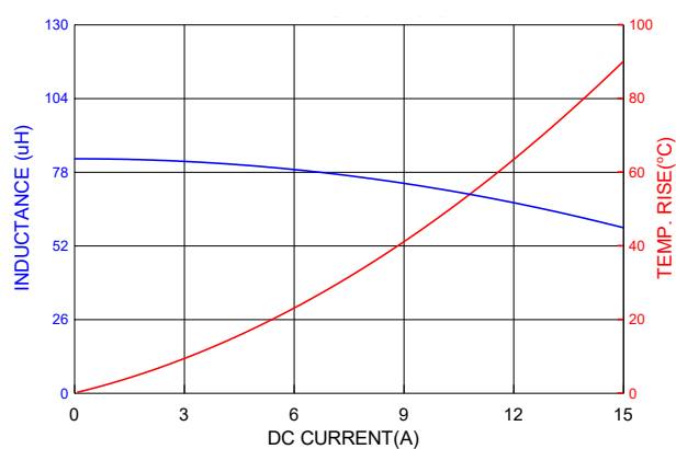
PIC1707HP820MF
