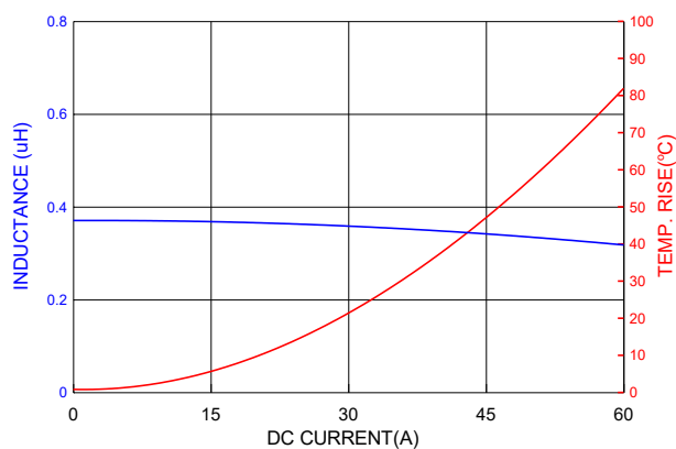
PIC1004HR36MF
