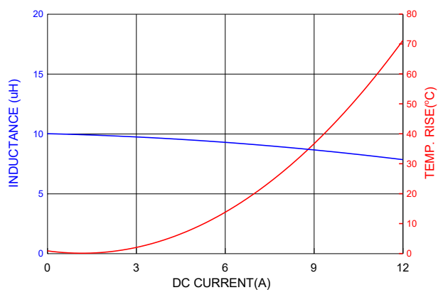
PIC1004H100MF
