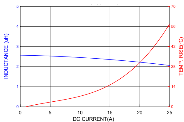
PIC1004H2R5MF
