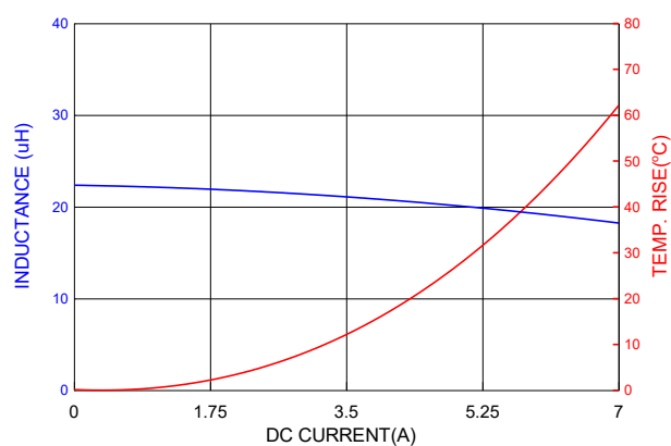
PIC1004H220MF
