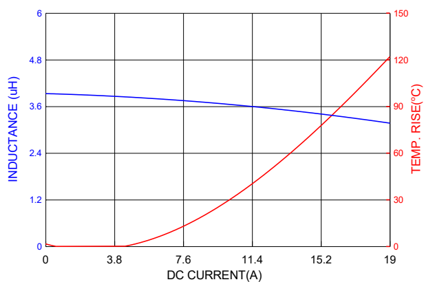
PIC1004H3R9MF
