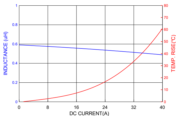
PIC1004HR56MF
