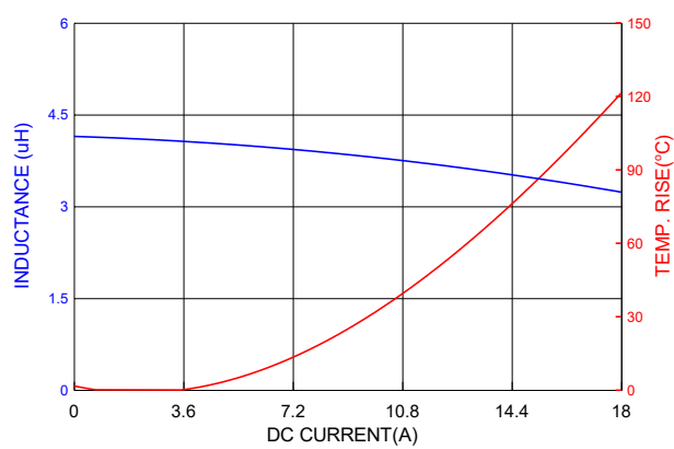
PIC1004H4R0MF
