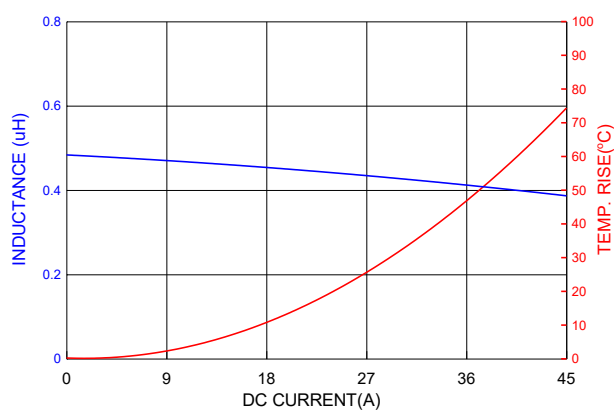
PIC1004HR45MF
