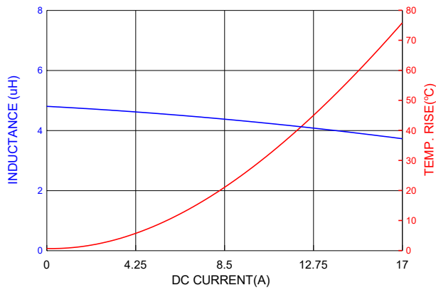
PIC1004H4R7MF
