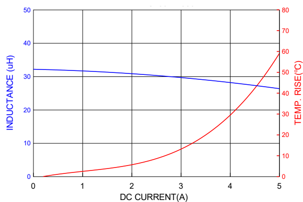
PIC1004H330MF
