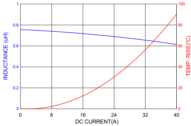
PIC1004HR75MF
