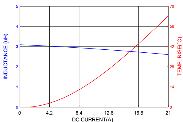
PIC1004H3R0MF
