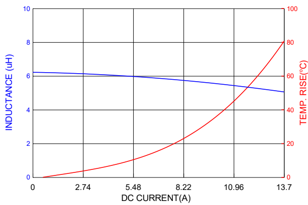
PIC1004H6R2MF
