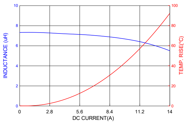
PIC1004H7R3MF
