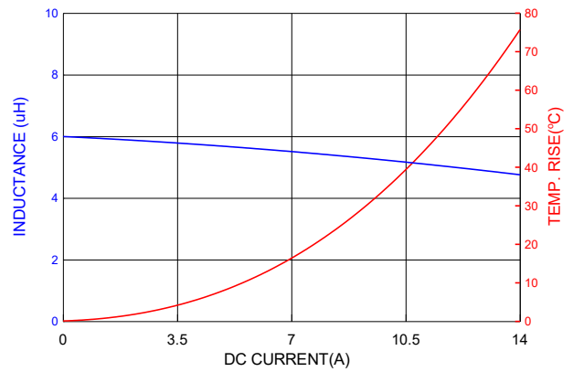
PIC1004H5R6MF
