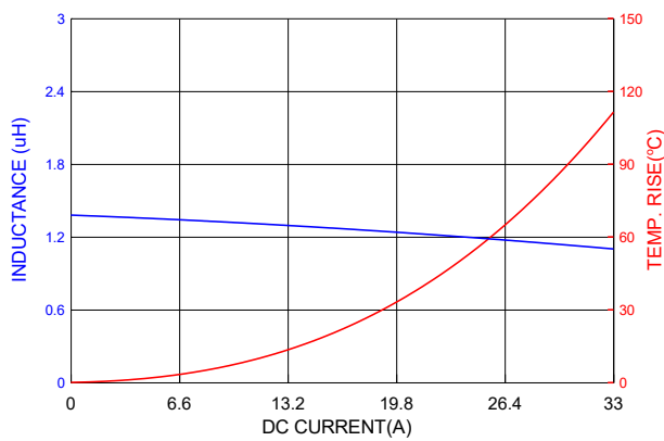
PIC1004H1R5MF
