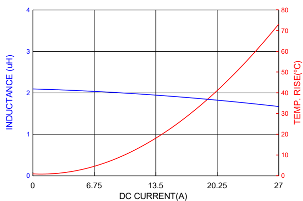
PIC1004H2R2MF
