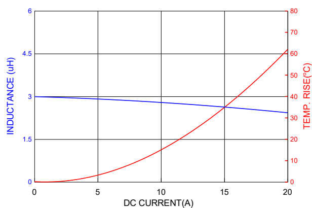
PIC1004H3R3MF
