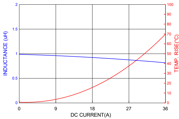
PIC1004H1R0MF
