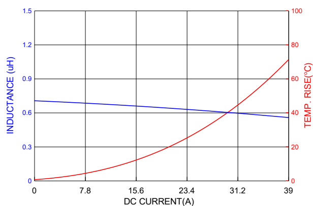
PIC1004HR68MF
