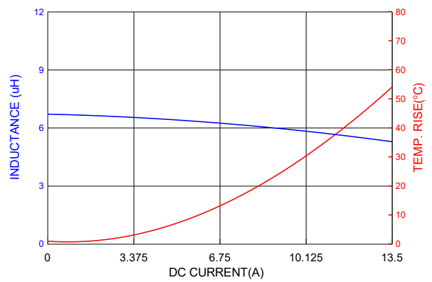
PIC1004H6R8MF
