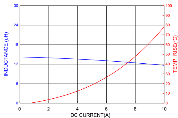
PIC1004H150MF
