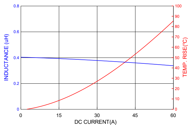
PIC1004HR39MF
