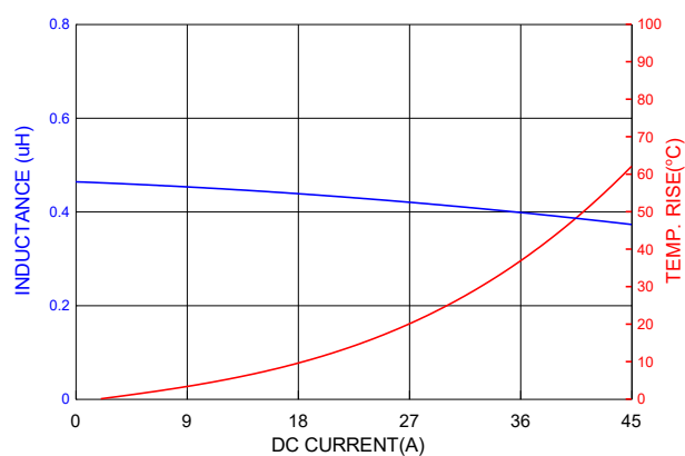
PIC1004HR47MF
