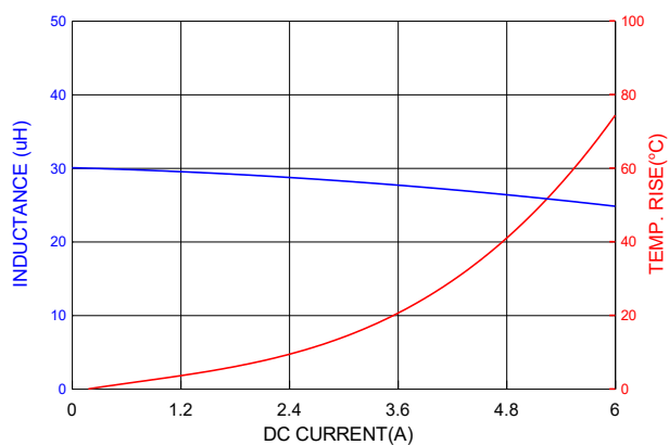
PIC1004H270MF
