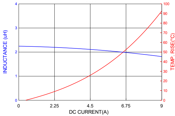
PIC0502HP2R2MF
