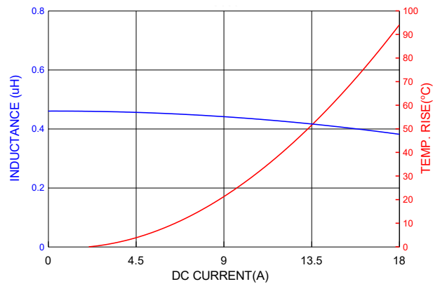
PIC0502HPR47MF
