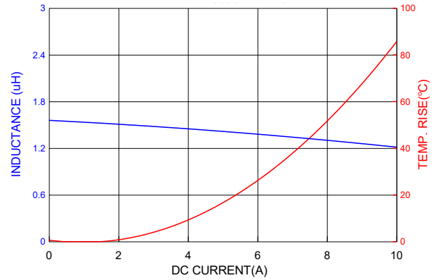
PIC0502HP1R5MF
