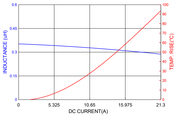
PIC0502HPR33MF
