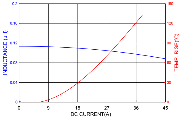
PIC0502HPR10YF
