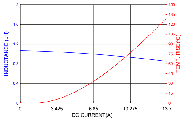
PIC0502HP1R0MF
