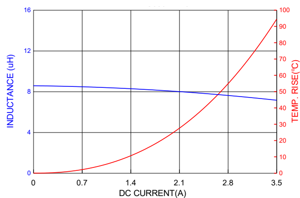
PIC0502HP8R2MF
