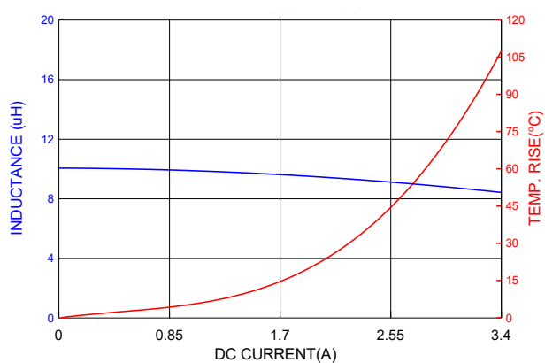
PIC0502HP100MF
