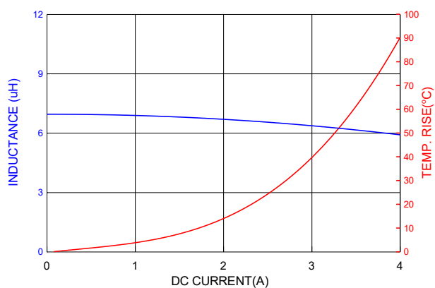
PIC0502HP6R8MF
