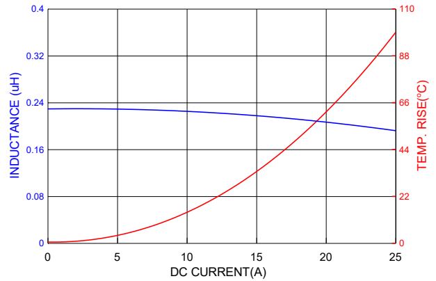
PIC0502HPR22MF
