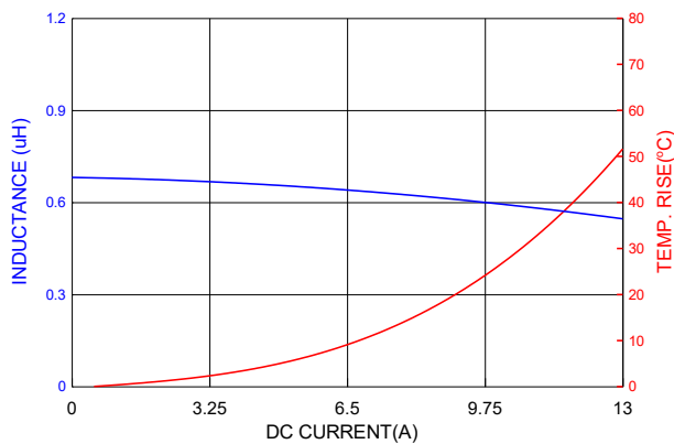
PIC0502HPR68MF
