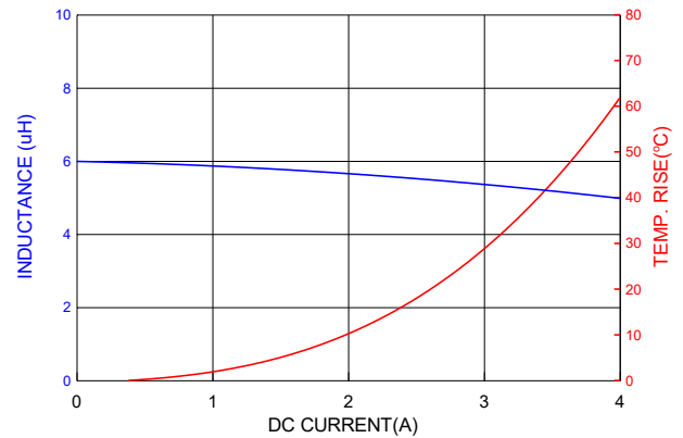
PIC0502HP5R6MF
