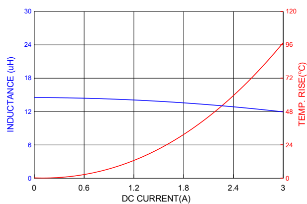
PIC0502HP150MF
