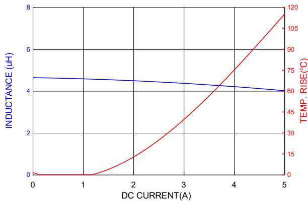
PIC0502HP4R7MF
