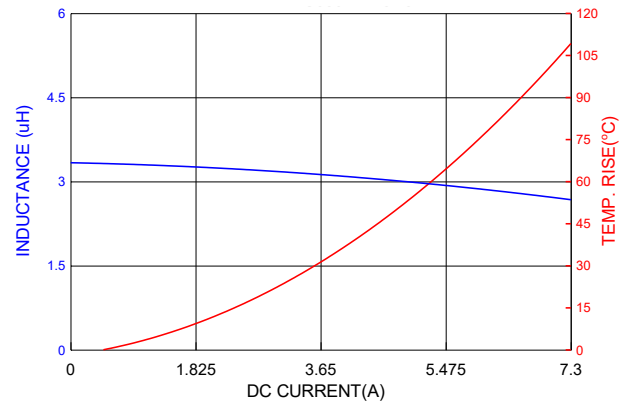
PIC0502HP3R3MF
