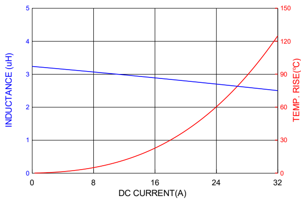
PICQ1205HP3R3MF
