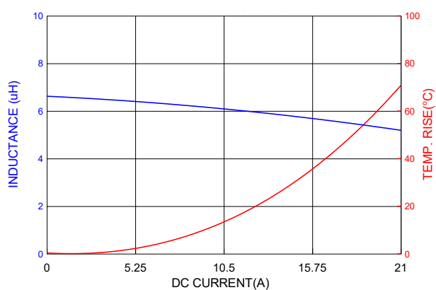
PICQ1205HP6R8MF
