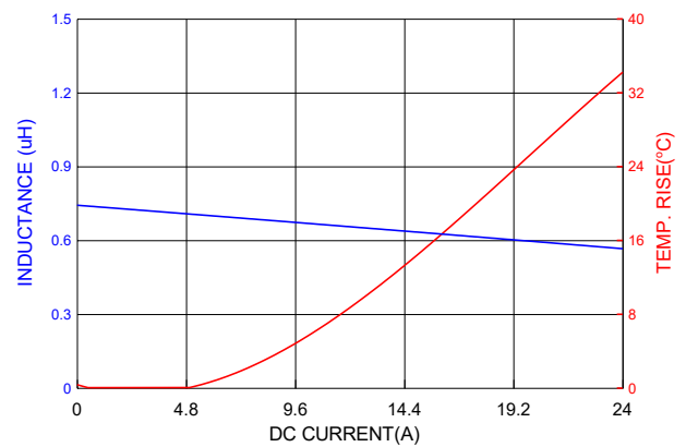
PICQ0604HR68MF
