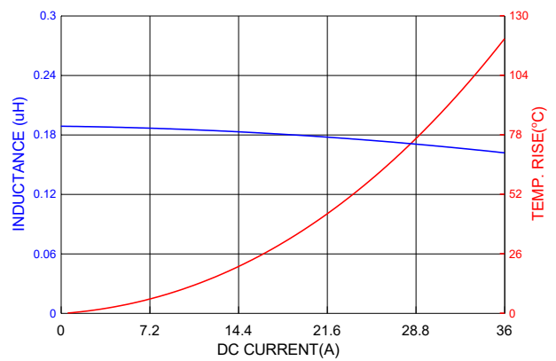
PICQ0602HR18YF
