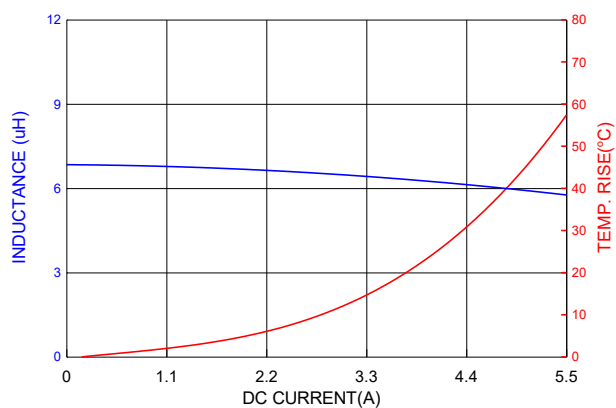
PICQ0602H6R8MF
