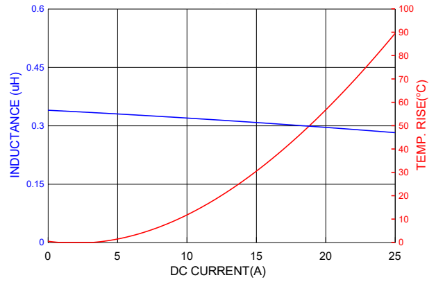
PICQ0602HR33MF
