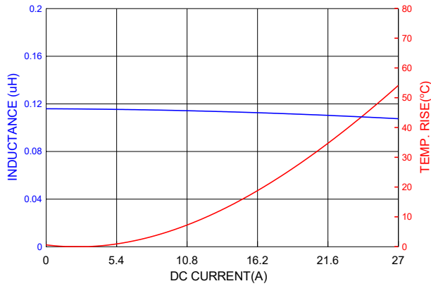
PICQ0503HR10YF
