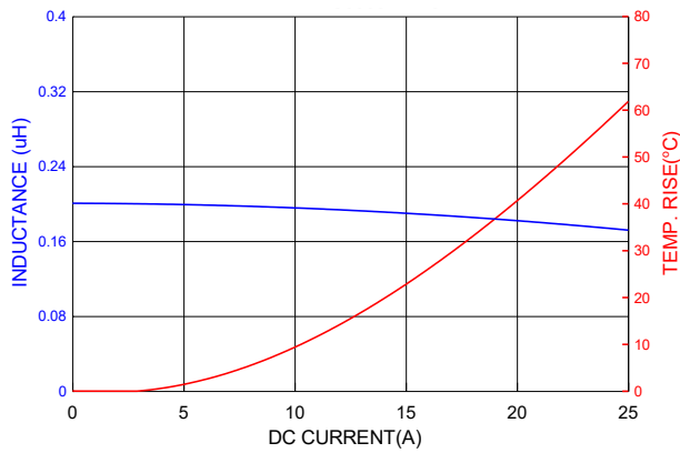
PICQ0503HR20YF
