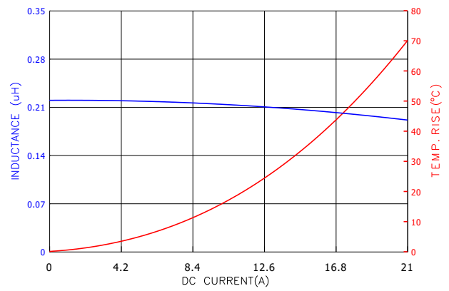
PICQ0503HR22MF
