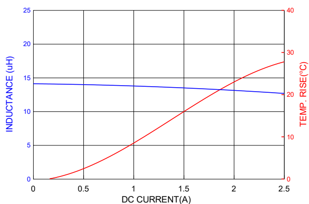
PICQ0503HP150MF
