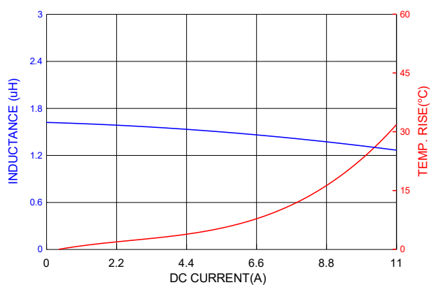
PICQ0503HP1R5MF
