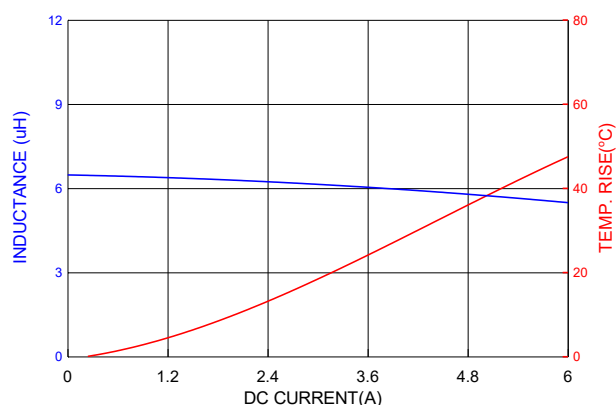
PICQ0503HP6R8MF
