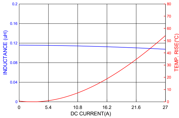
PICQ0503HPR10YF
