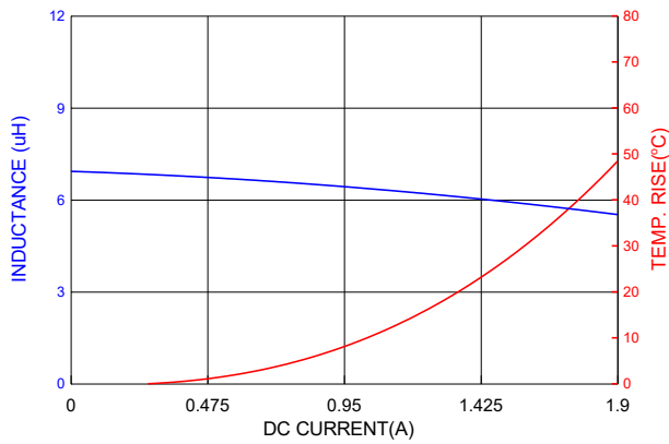
PICQ0412HP6R8MF
