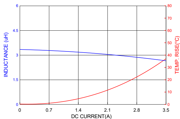
PICQ0412HP3R3MF
