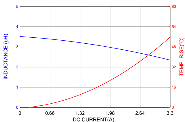
PICQ0318H3R3MF
