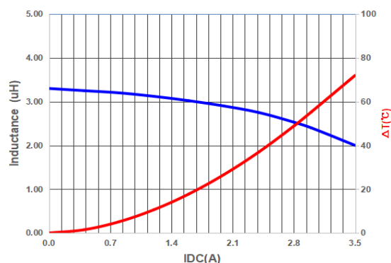
PIM252012A3R3M
