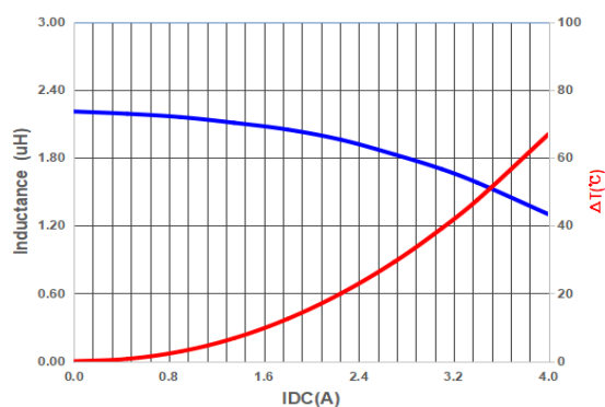
PIM252012A2R2M
