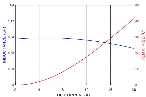
PIAQ0624SR82MN
