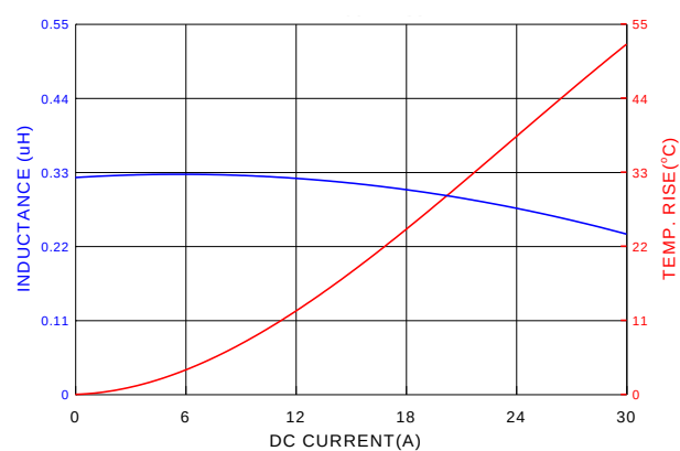
PIAQ0624SR33MN
