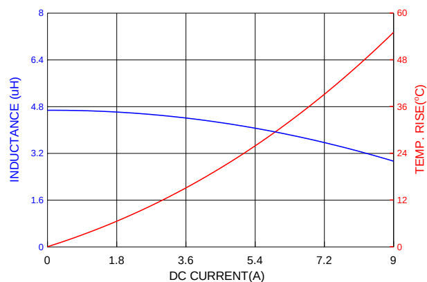
PIAQ0624S4R7MN
