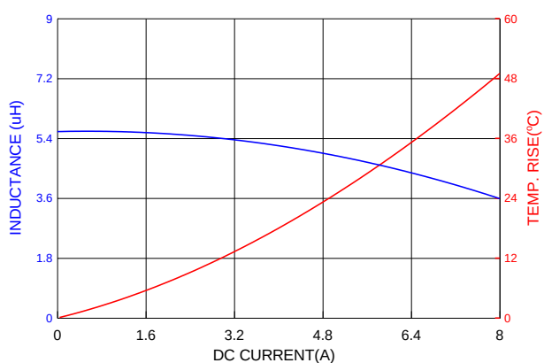
PIAQ0624S5R6MN
