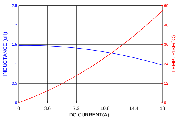
PIAQ0624S1R5MN
