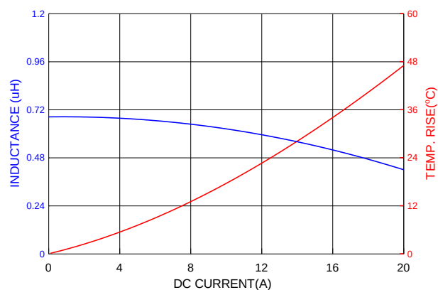
PIAQ0624SR68MN
