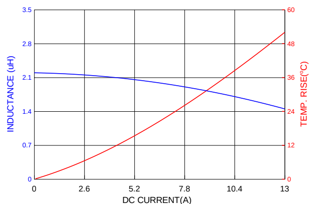
PIAQ0624S2R2MN
