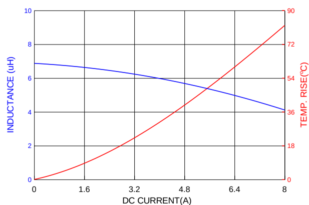
PIAQ0624S6R8MN
