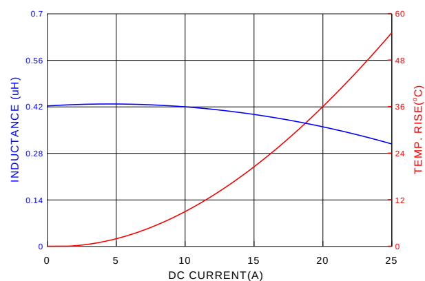
PIAQ0624SR36MN
