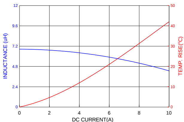
PIAQ0605S6R8MN
