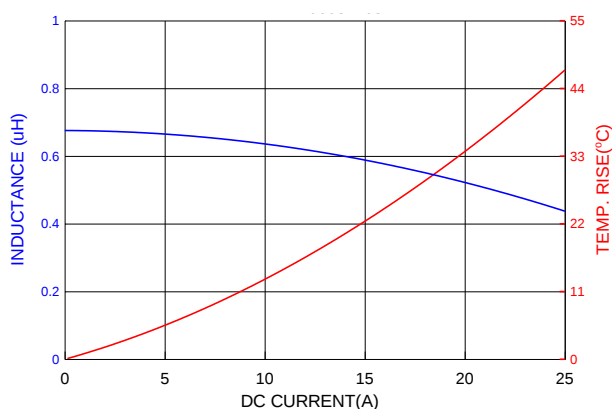
PIAQ0605SR68MN
