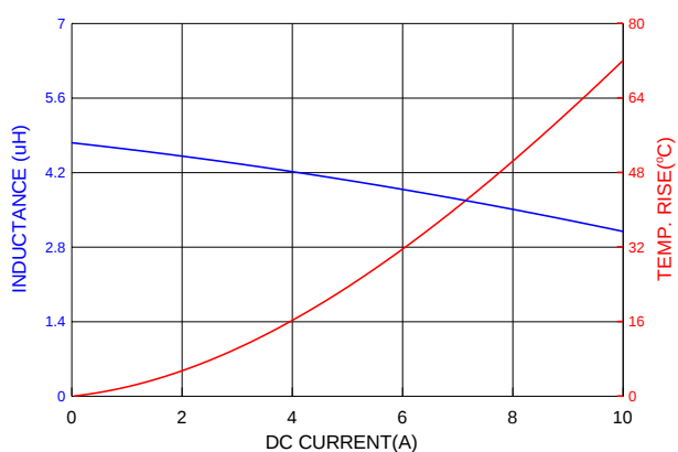
PIAQ0603S4R7MN
