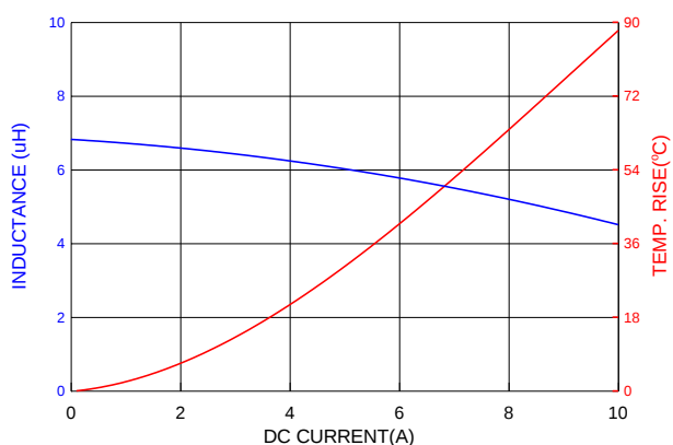
PIAQ0603S6R8MN
