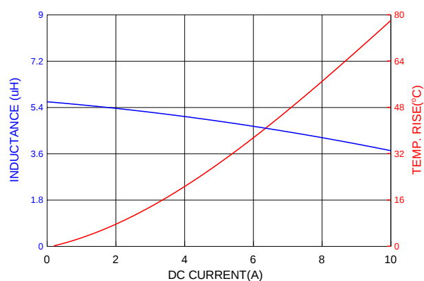
PIAQ0603S5R6MN
