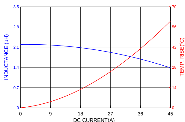
PIA1707SP2R2MN
