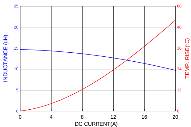
PIA1707SP150MN
