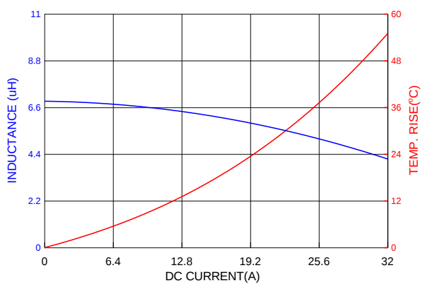
PIA1707SP6R8MN
