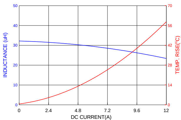
PIA1265SP330MN
