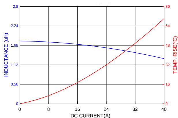
PIA1265SP1R8MN
