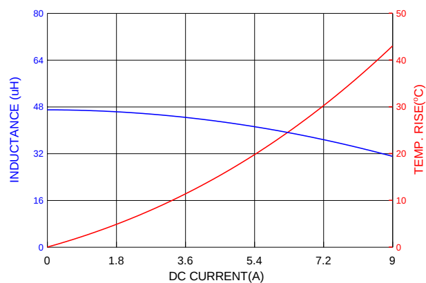
PIA1265SP470MN
