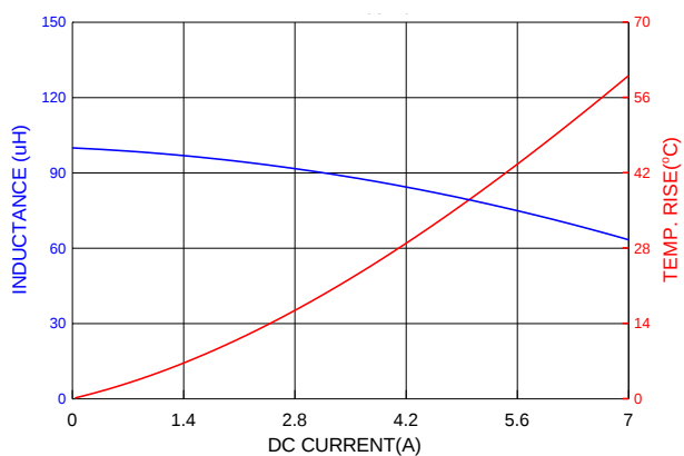
PIA1265SP101MN
