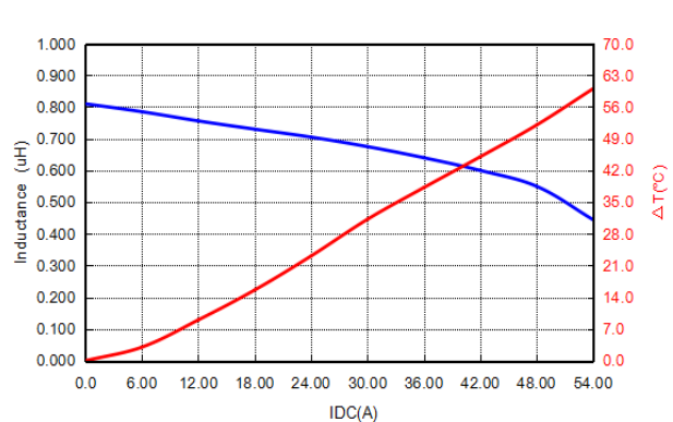
PIA1265SPR82MN
