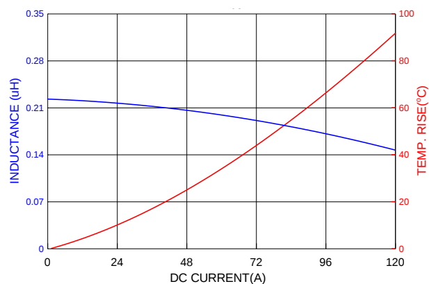
PIA1265SPR22MN
