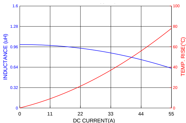
PIA1265SP1R0MN
