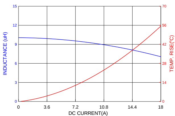
PIA1265SP100MN
