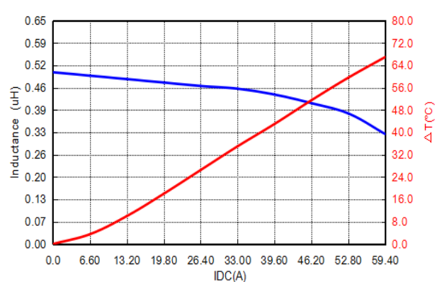
PIA1265SPR56MN
