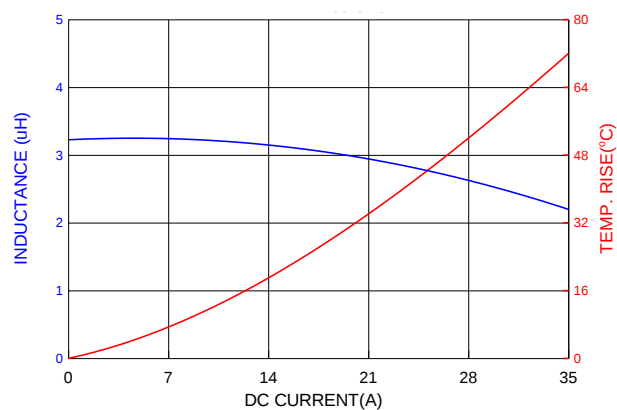
PIA1265SP3R3MN
