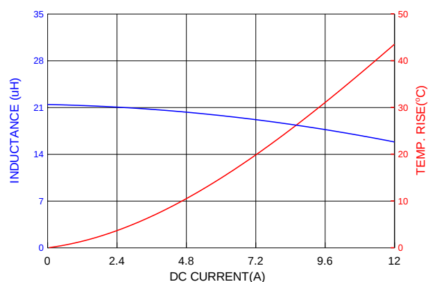
PIA1265SP220MN
