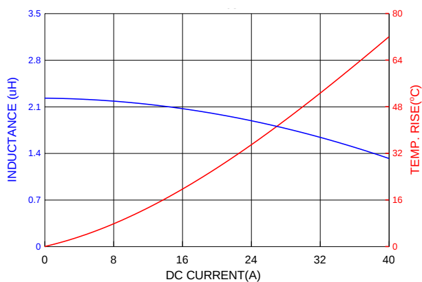
PIA1265SP2R2MN
