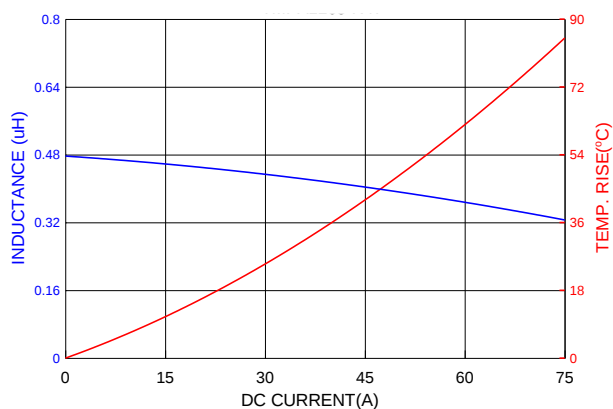
PIA1265SPR47MN
