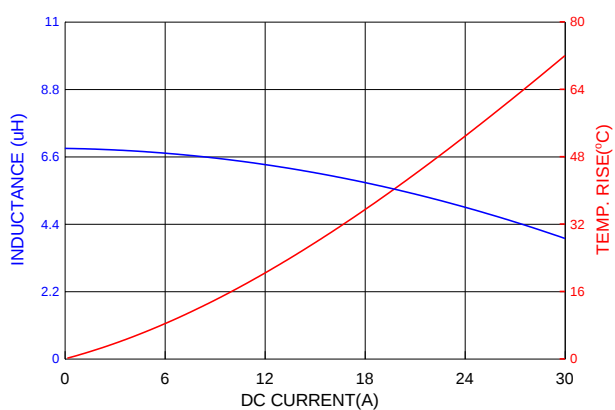
PIA1265SP6R8MN
