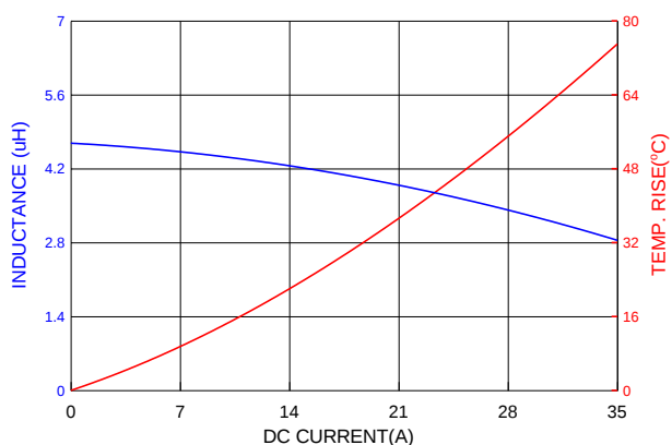
PIA1265SP4R7MN
