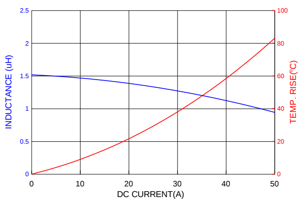
PIA1265SP1R5MN
