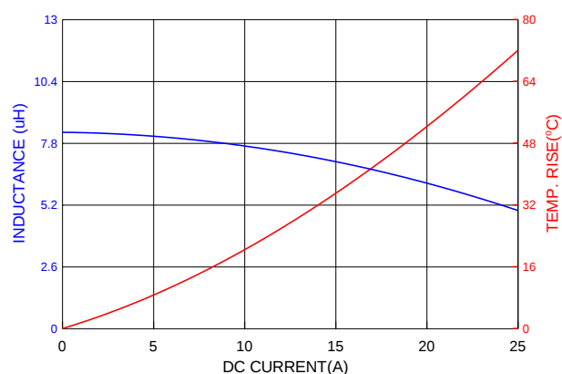
PIA1265SP8R2MN
