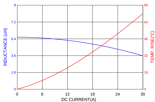
PIA1265SP5R6MN
