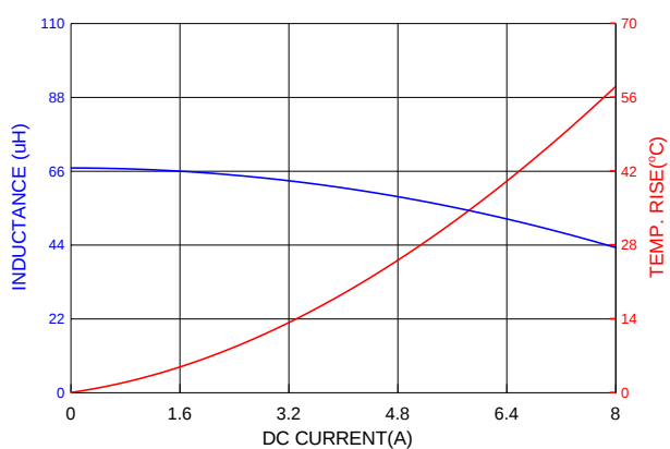
PIA1265SP680MN
