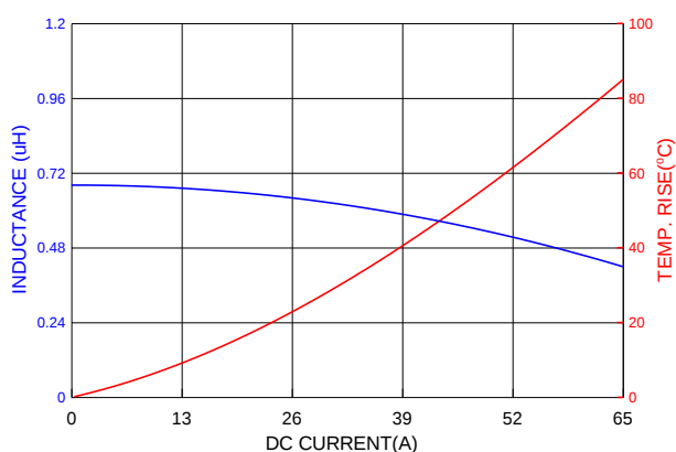
PIA1265SPR68MN
