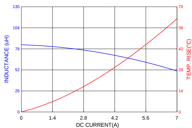
PIA1265SP820MN
