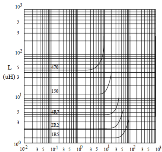
@ INDUCTANCE VS. FREQUENCY RESPONSE CURVE
