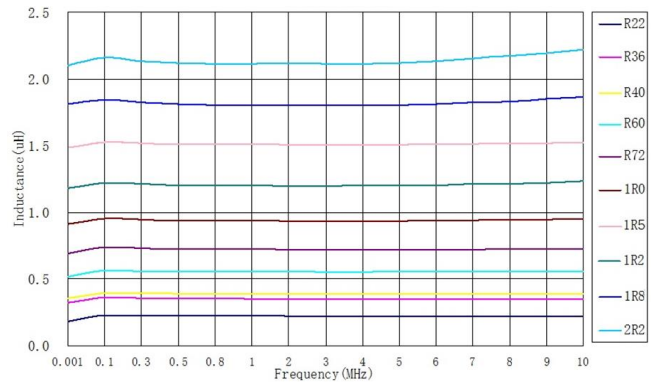
PIF0402A Series
