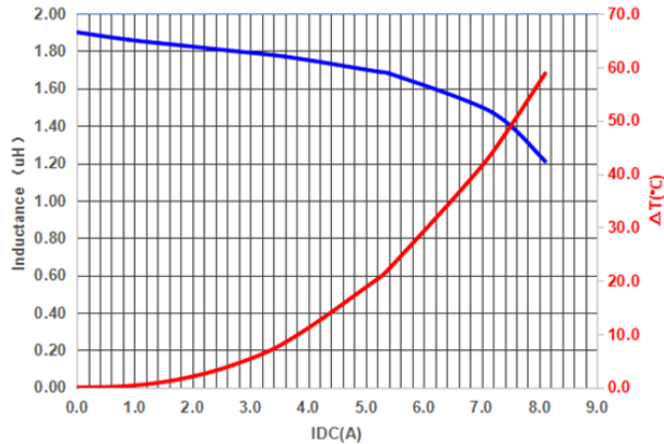
PIF0402A1R8MN
