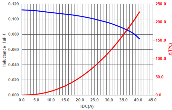
PIF0402AR10MN
