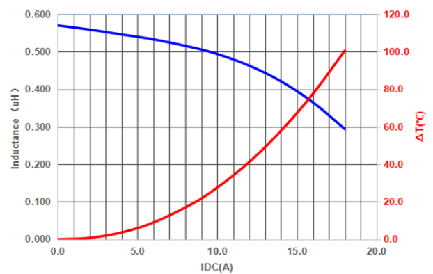
PIF0402AR56MN
