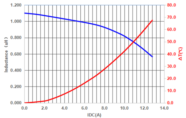
PIF0402A1R0MN
