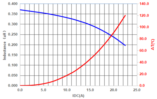
PIF0402AR36MN
