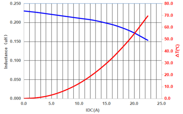
PIF0402AR22MN
