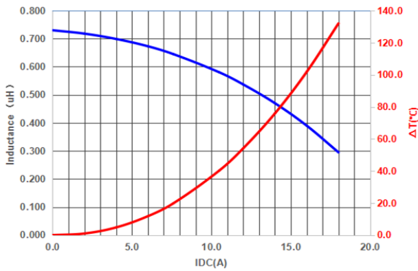
PIF0402AR72MN
