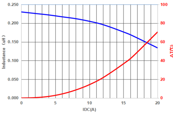
PIF0402AR33MN
