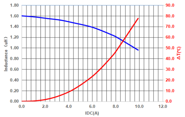
PIF0402A1R5MN
