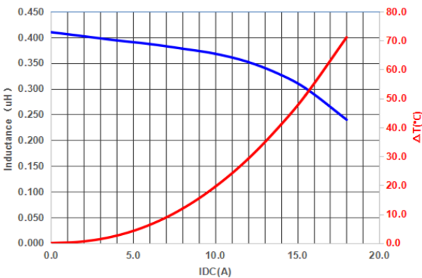
PIF0402AR40MN
