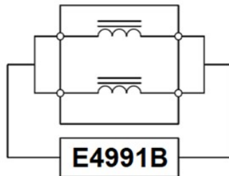
Common mode
