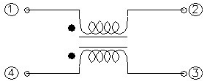
Common mode
