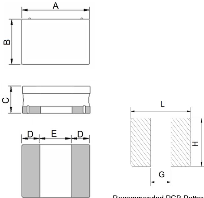
Recommended PCB Pattern
