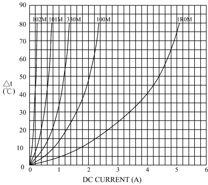
TEMPERATURE RISE vs. DC CURRENT
