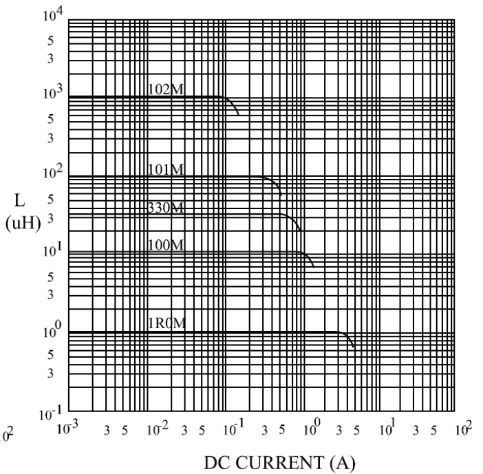
INDUCTANCE vs. DC CURRENT
