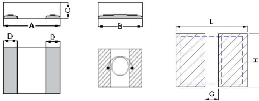
Recommended PCB Pattern
