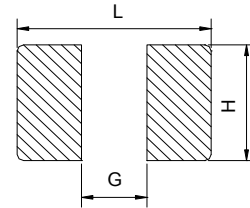
Recommended PC Board Pattern
