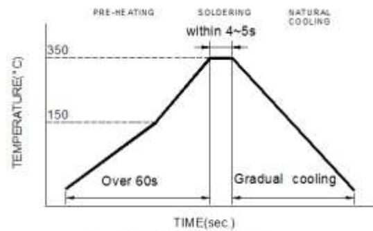
Iron Soldering times: 1 times max.
