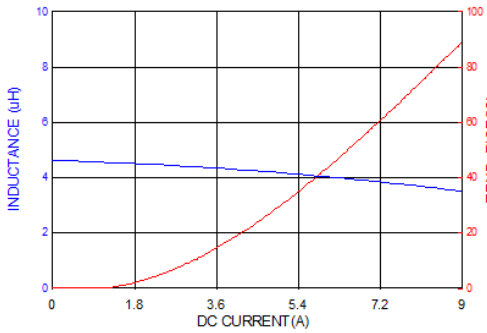
PICQ0624H4R7MF
