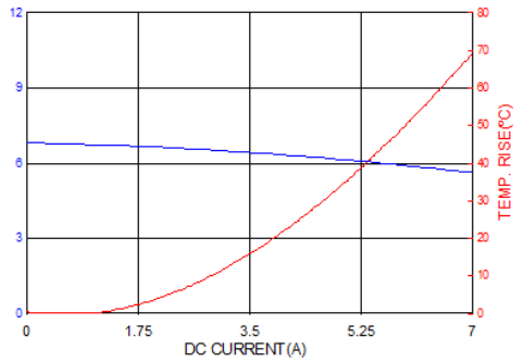
PICQ0624H6R8MF
