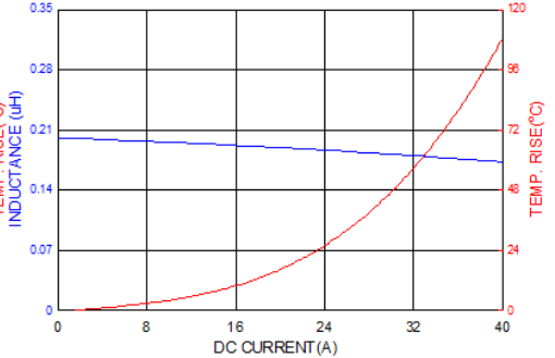
PICQ0624HR20MF
