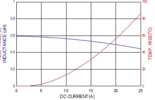
PICQ0624HR60MF
