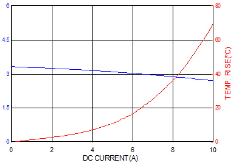
PICQ0624H3R3MF
