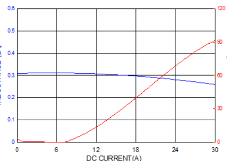
PICQ0624HR33MF
