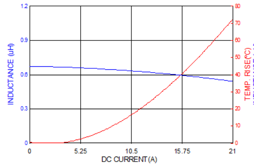
PICQ0624HR68MF
