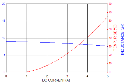
PICQ0624H100MF
