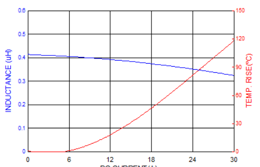
PICQ0624HR36MF
