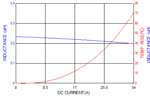
PICQ0624HR22MF
