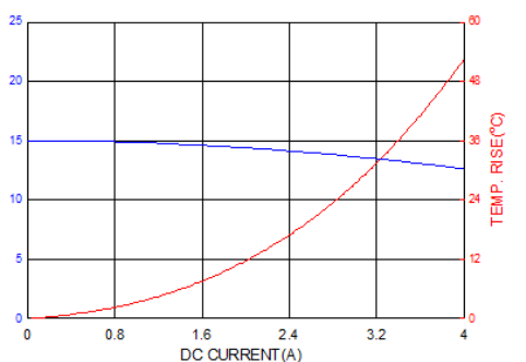
PICQ0624H150MF
