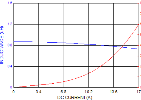
PICQ0624HR82MF
