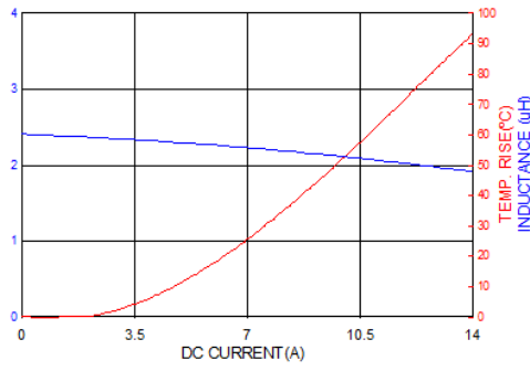
PICQ0624H2R2MF
