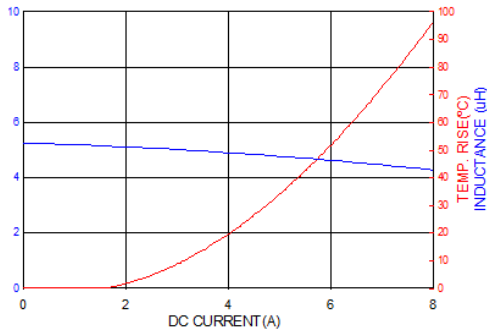
PICQ0624H5R6MF
