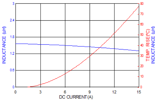
PICQ0624H1R5MF
