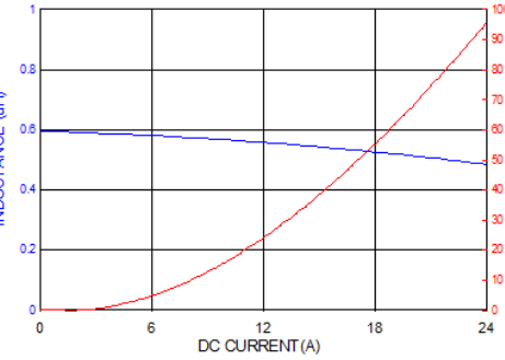
PICQ0624HR56MF
