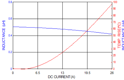
PICQ0624HR47MF
