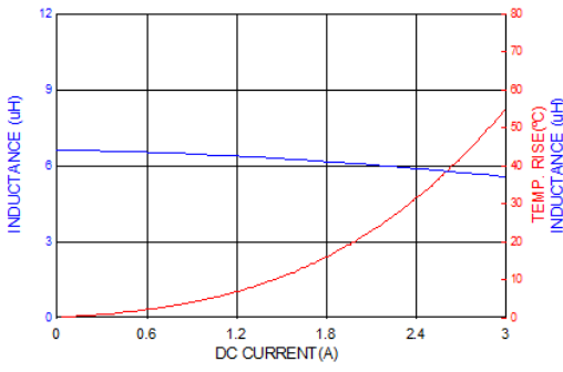
PICQ0612H6R8MF
