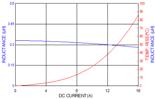
PICQ0612HR33MF
