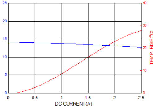
PICQ0503HP150MF
