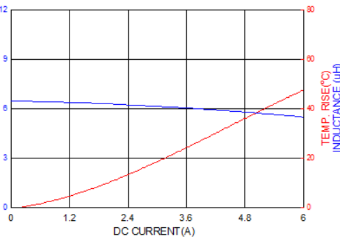
PICQ0503HP6R8MF
