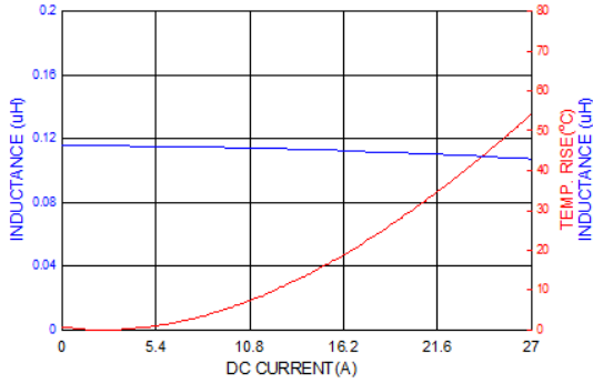
PICQ0503HPR10YF
