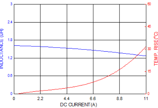
PICQ0503HP1R5MF
