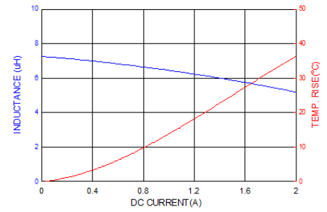
PICQ0312H6R8MF
