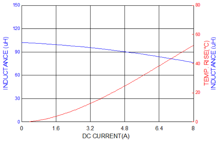
PIC1206HP101MF
