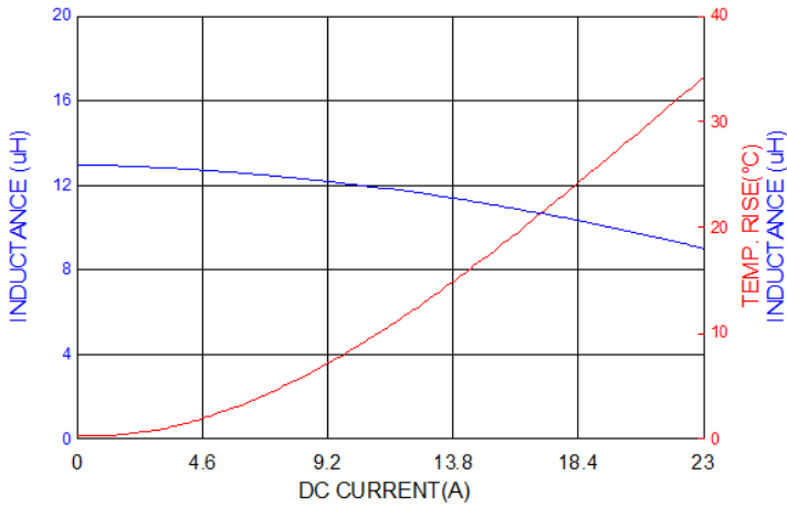
PIC1206HP120MF
