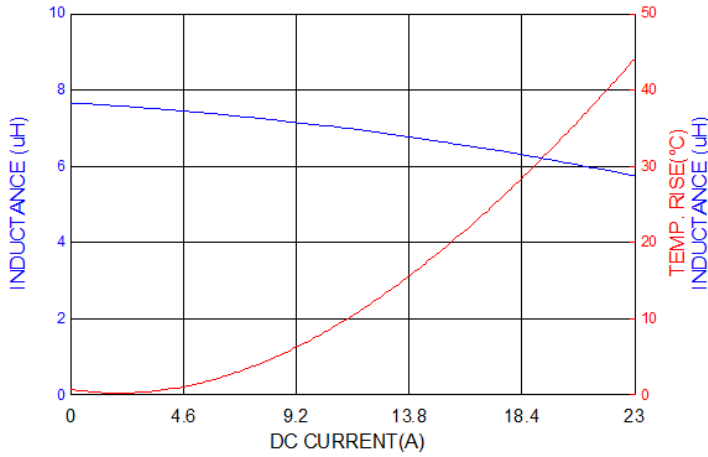
PIC1206HP8R2MF
