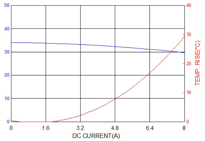
PIC1206HP330MF
