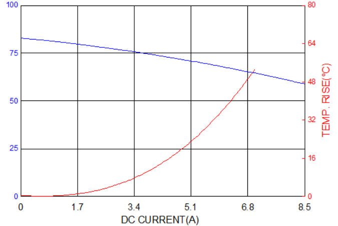
PIC1206HP820MF
