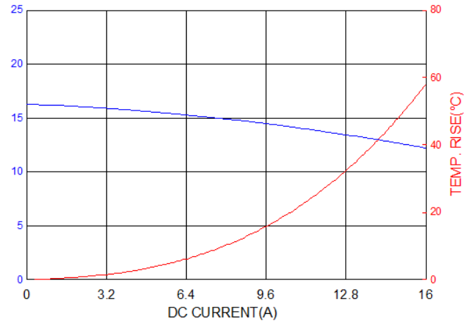
PIC1206HP150MF
