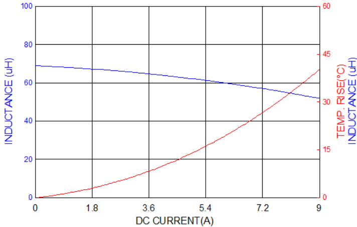
PIC1206HP680MF
