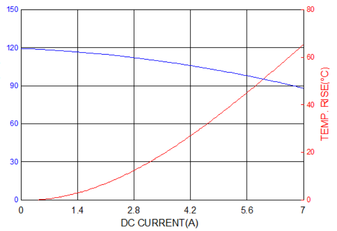
PIC1206HP121MF
