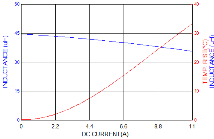
PIC1206HP470MF
