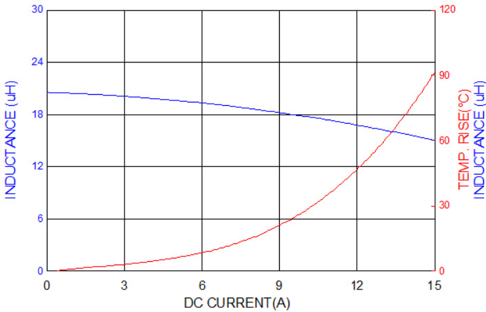
PIC1206HP180MF
