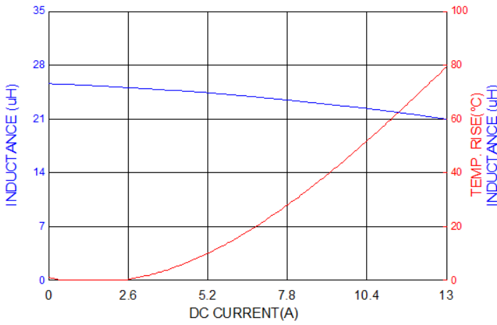
PIC1206HP270MF
