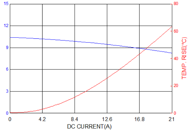
PIC1206HP100MF
