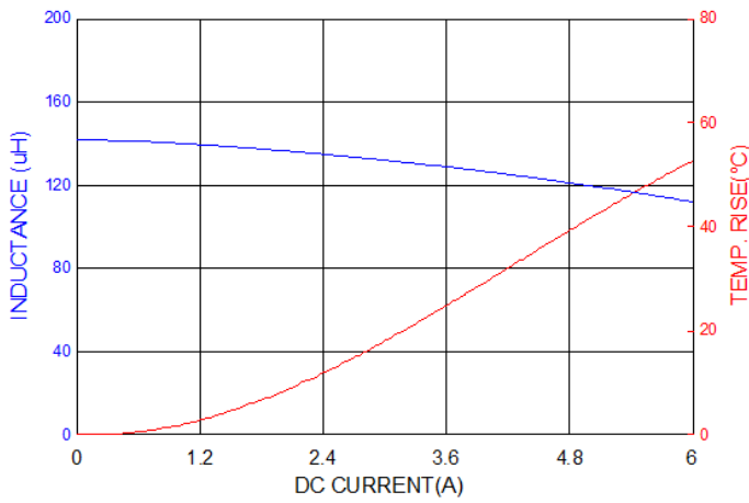
PIC1206HP151MF
