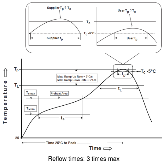
Fig.1 IR Soldering Reflow
